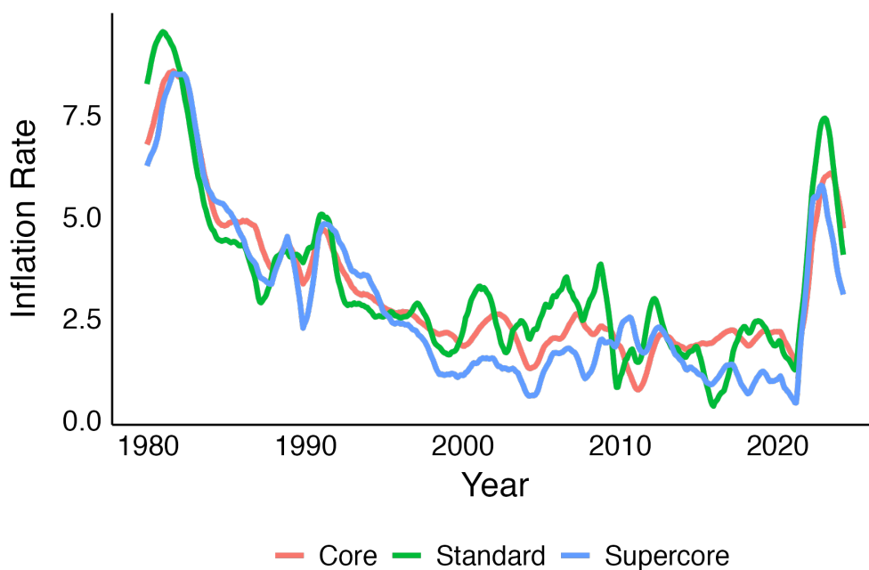
Figure 3: Headline, core, and supercore inflation for the aggregate smoothed with a twelve-month rolling average.
